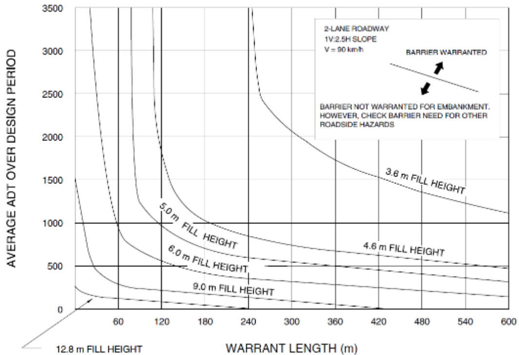
Figure 12: Cost-Effective Embankment Warrants Based on Traffic Speeds and Volumes, Slope and Length of Slope
