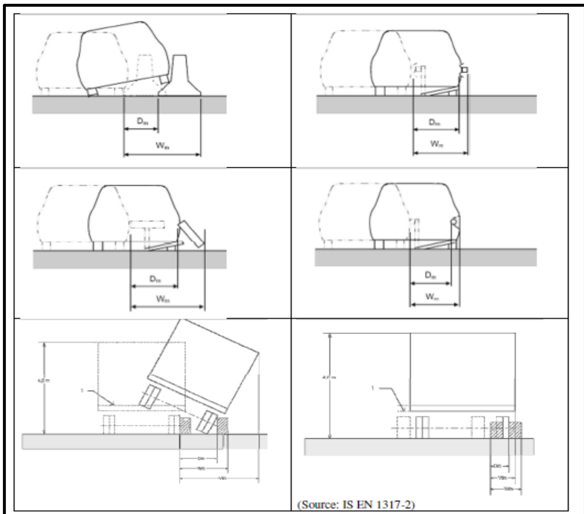
Figure 4: Working Widths and Deflection
