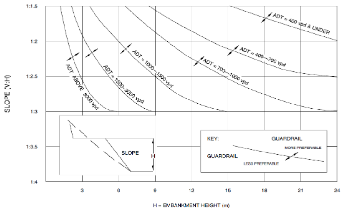
Figure 11: Design Chart for Embankment Warrants Based on Fill Height, Slope and Traffic Volume
