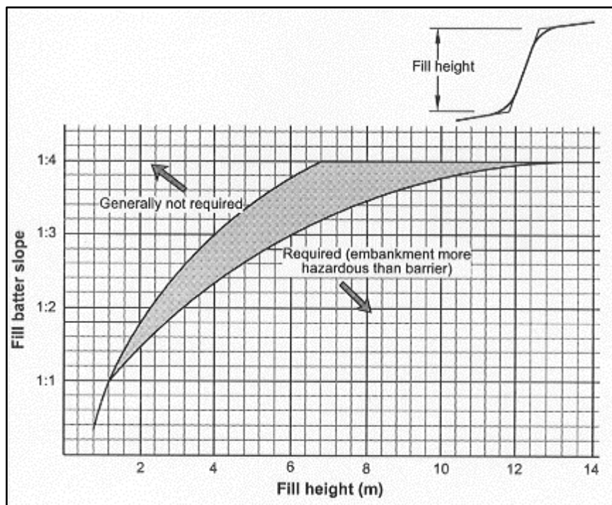
Figure 10: Warrants for the Use of Roadside Barriers
