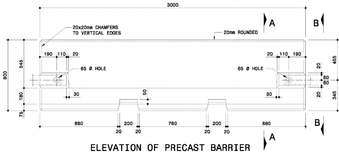
Figure 16: F-shape Precast Concrete Barriers (800 mm High Module)
