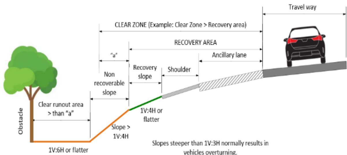
Figure 2: Roadside Terms Definitions
